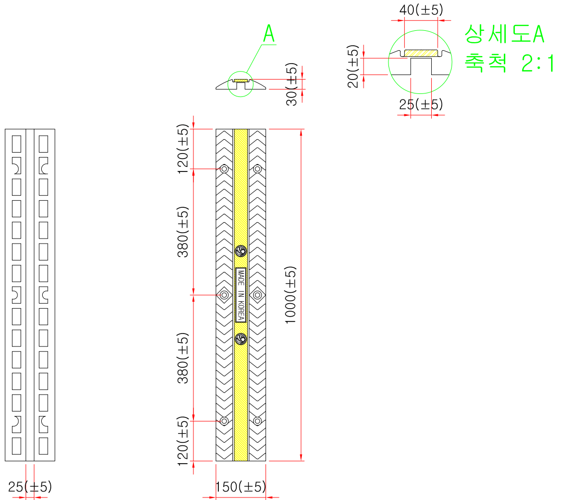
SIDE ELEVATION SCALE : NONE
